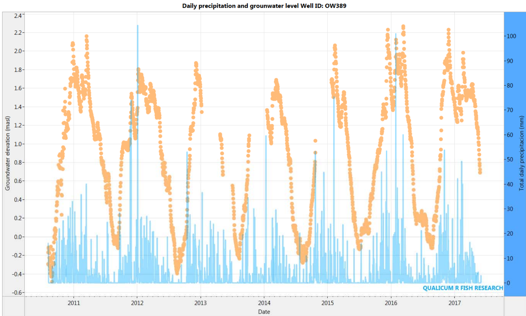
Figure 7. OW389: Daily groundwater levels compared to total daily precipitation (2010-2016)
