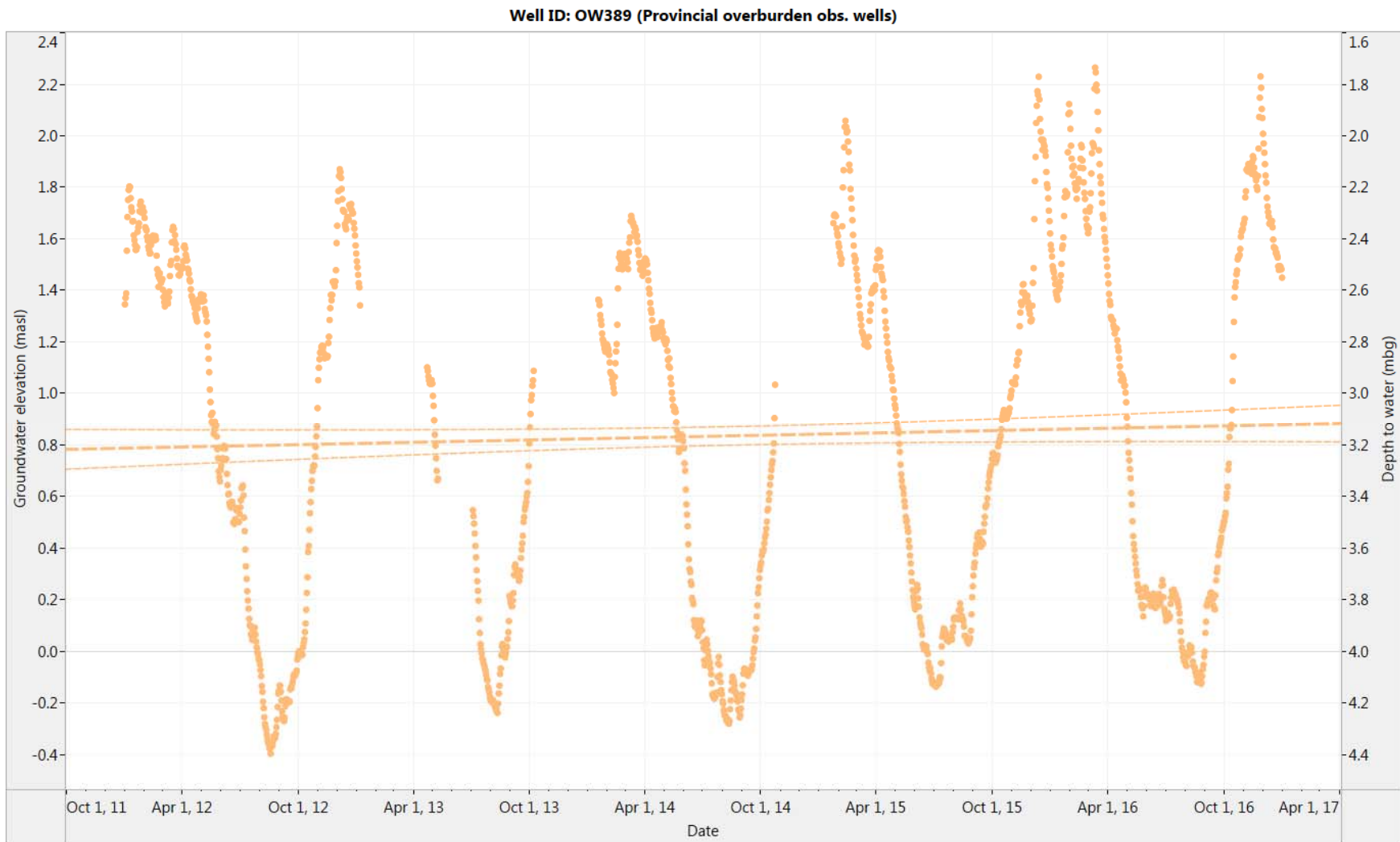
Figure 4. OW389: Water level and trend line estimation for the last five years (2012-2016)
