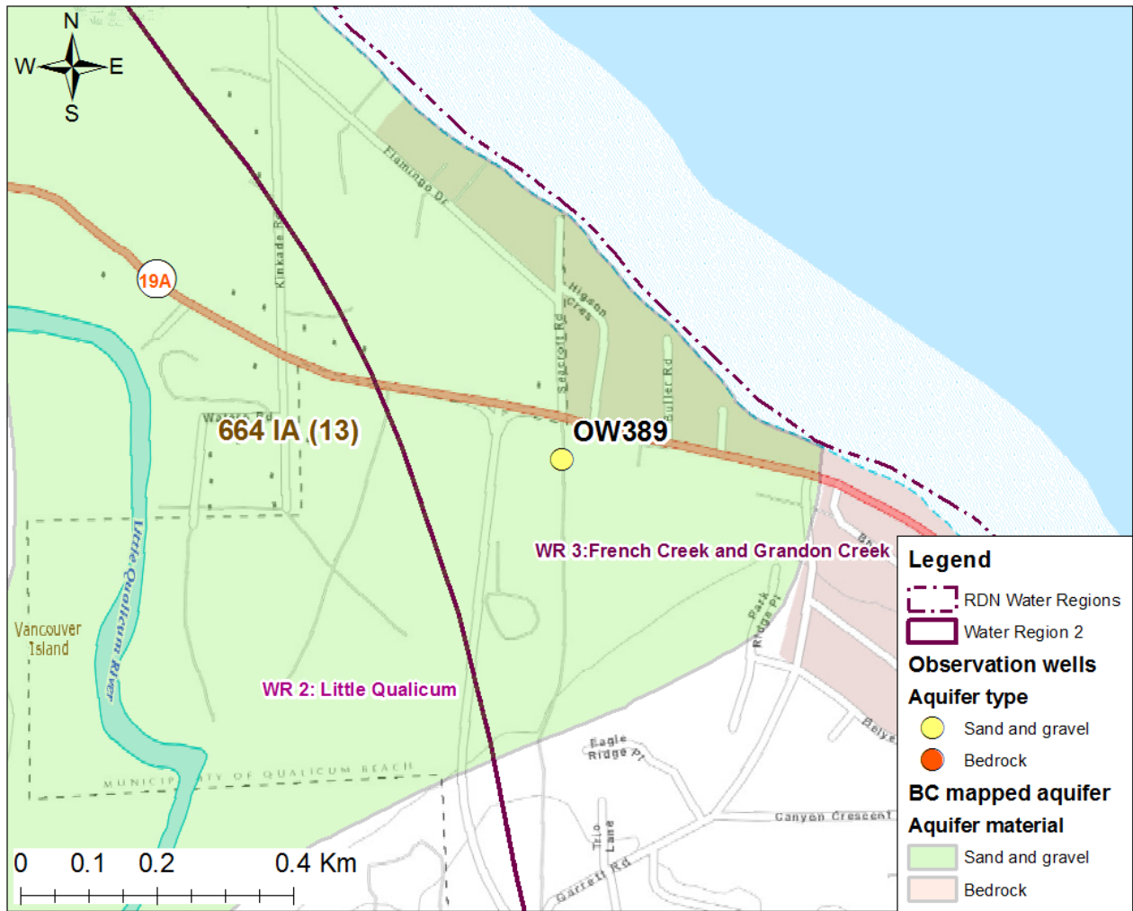
Figure 2. Location of observation well OW389
