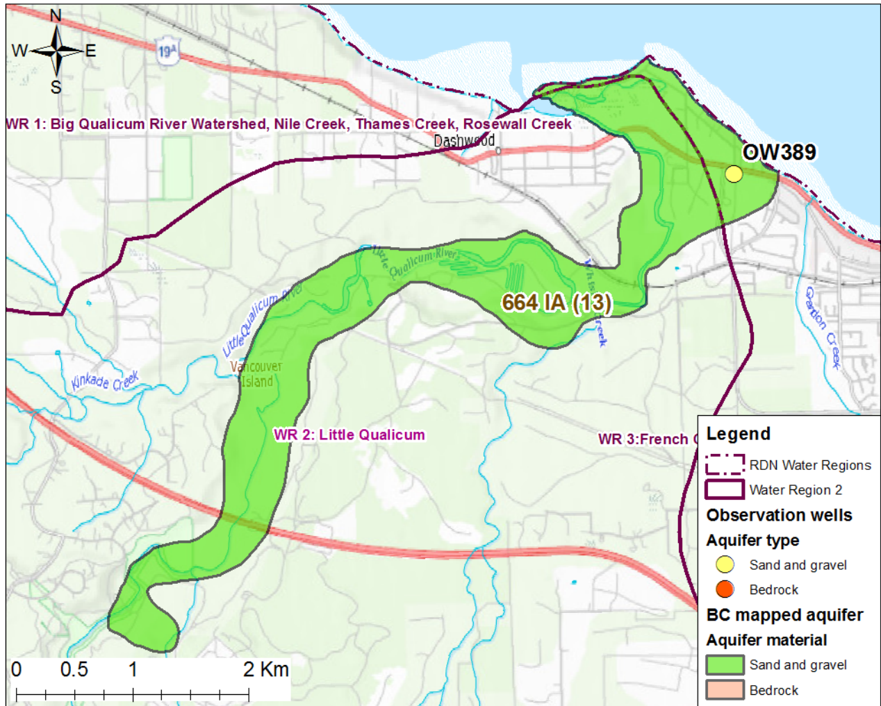
Figure 1. Location of mapped aquifer and observation well
