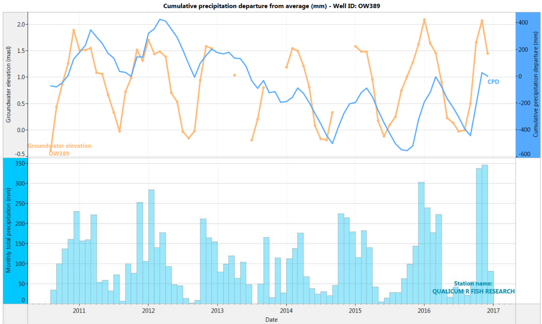
Figure 6. OW389: Month end groundwater levels compared to cumulative precipitation departure curve and total monthly precipitation (2010-2016)
