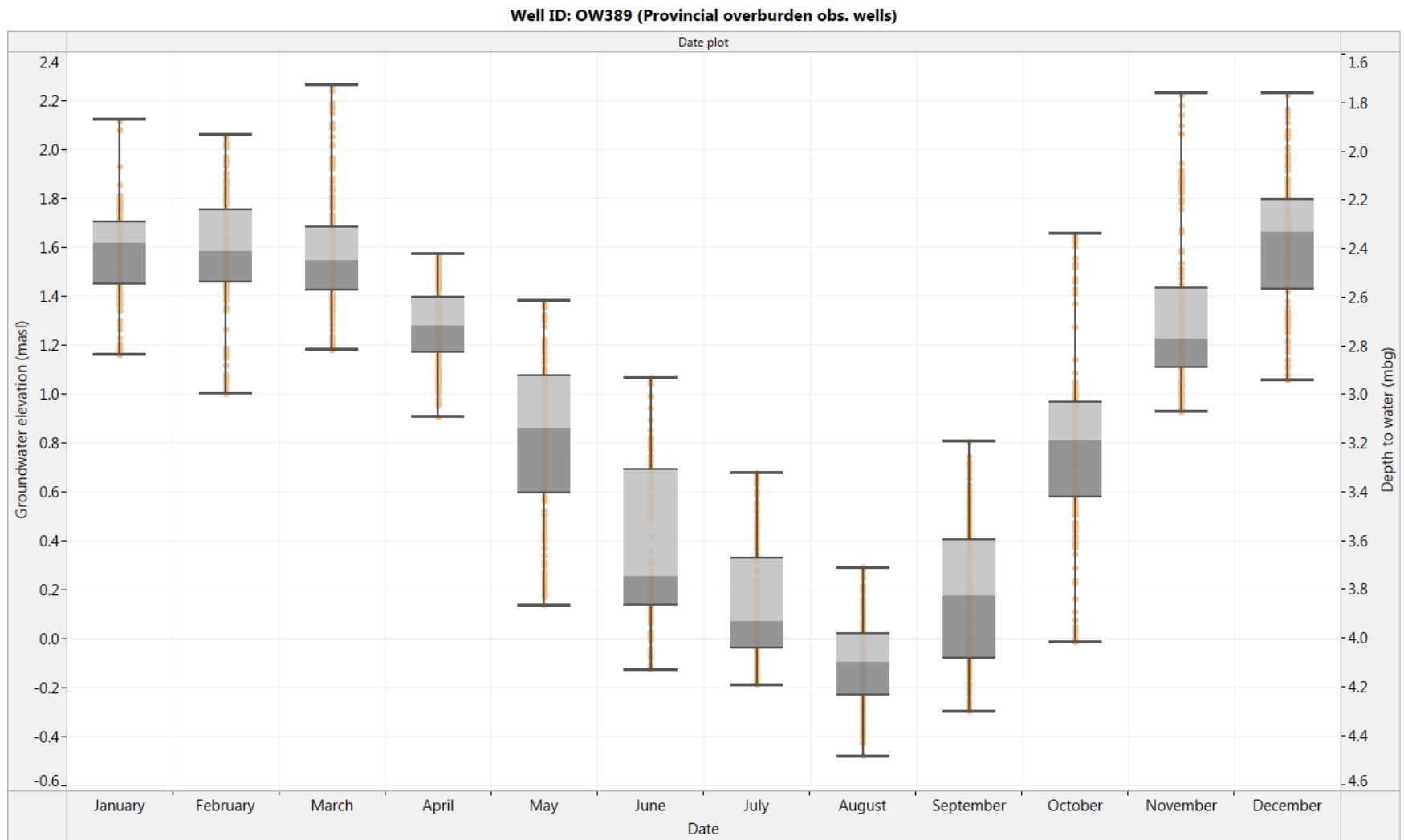
Figure 5. OW389: Box and Whisker diagram for historical monthly groundwater level fluctuation (2010-2016)
