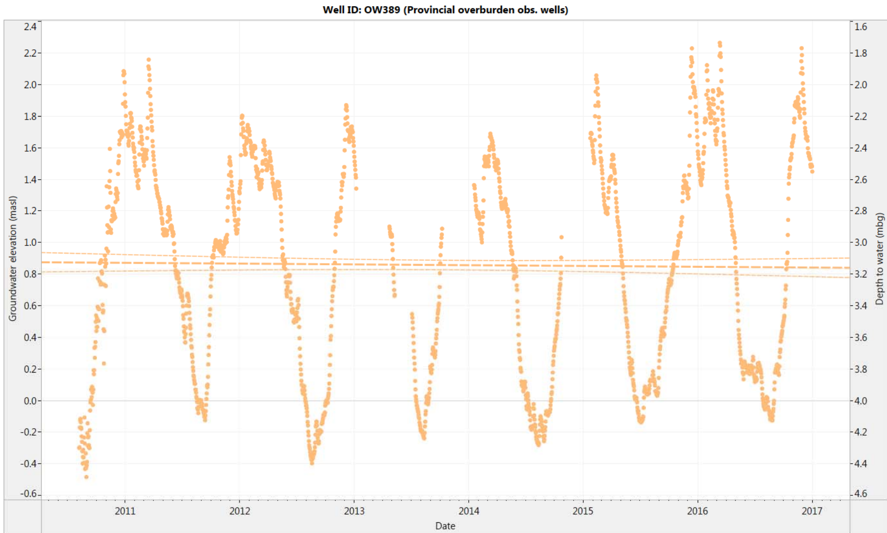
Figure 3. OW389: Historical daily water level (2010-2016) and trend line estimation (2010-2016)
