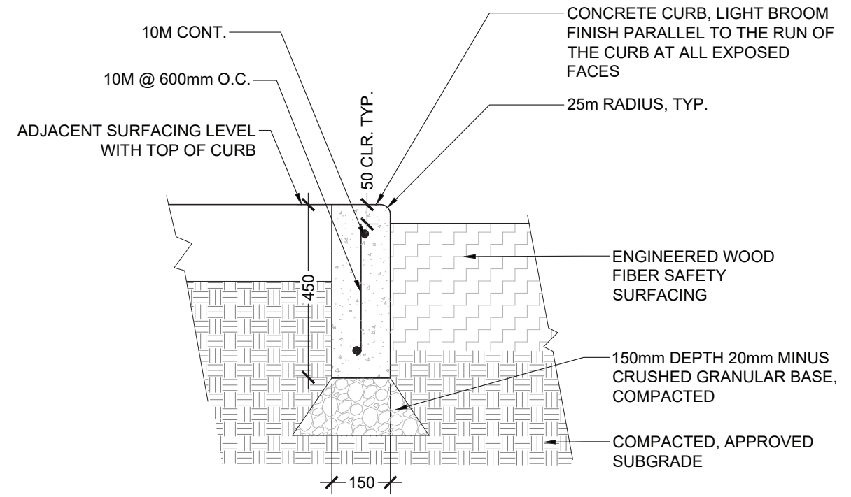
CONCRETE CURB DETAIL (PROVISIONAL ITEM)
