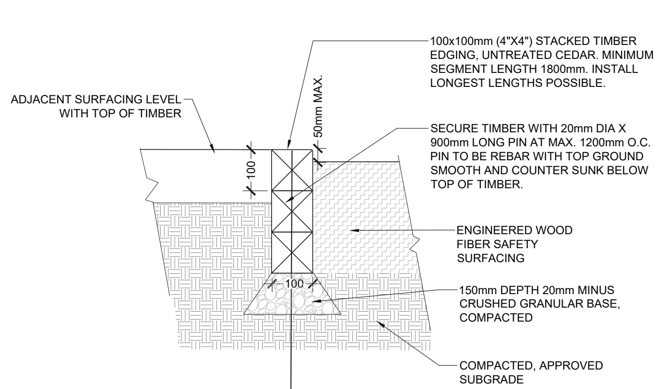
TIMBER BORDER DETAIL
