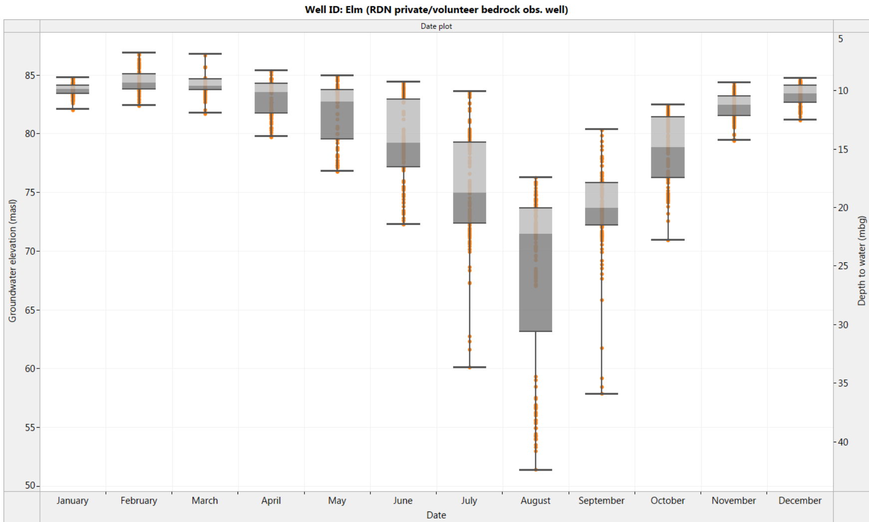
Figure 7. Elm: Box and Whisker diagram for historical monthly groundwater level fluctuation (2013-2016)
