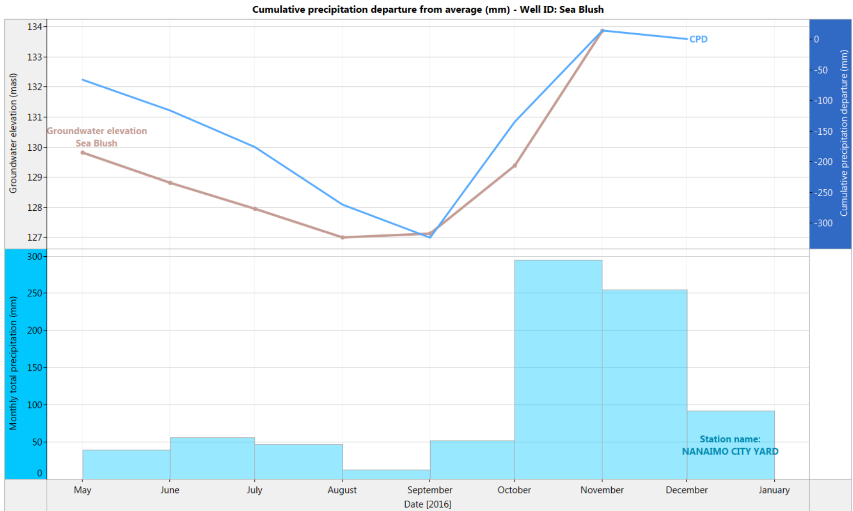
Figure 12. Sea Blush: Month end groundwater levels compared to cumulative precipitation departure curve and total monthly precipitation (2016)
