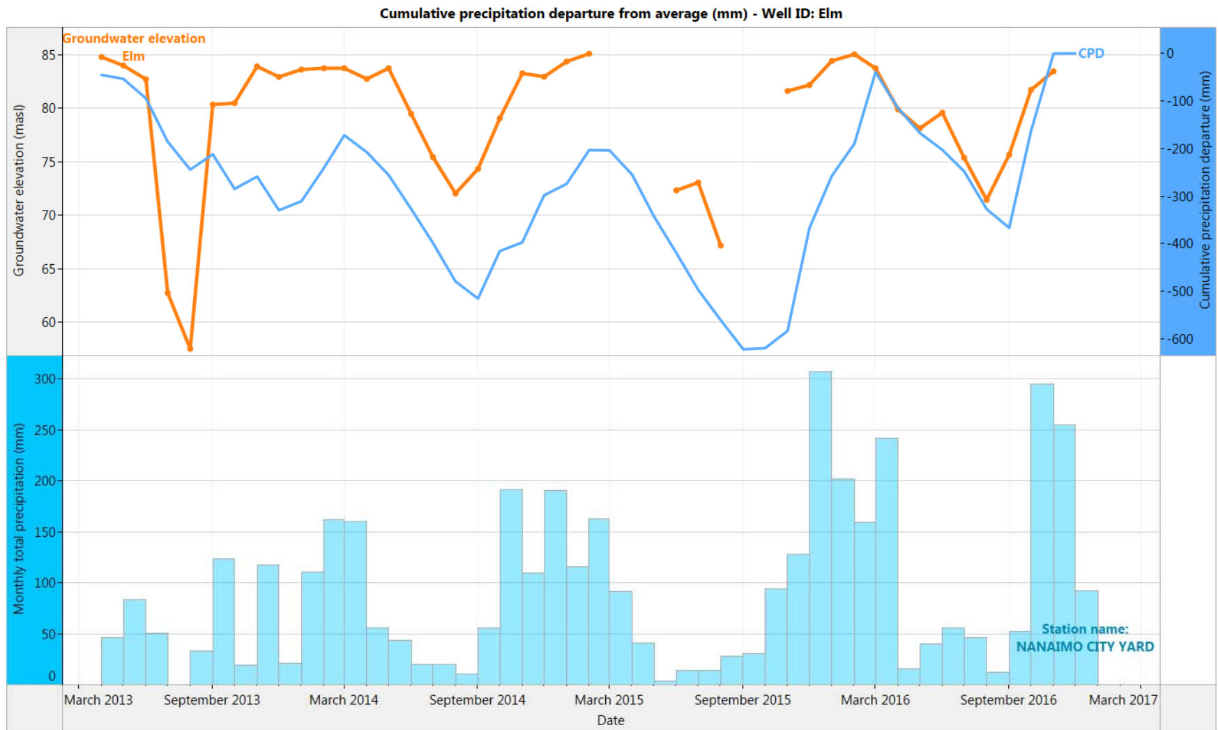
Figure 10. Elm: Month end groundwater levels compared to cumulative precipitation departure curve and total monthly precipitation (2013-2016)
