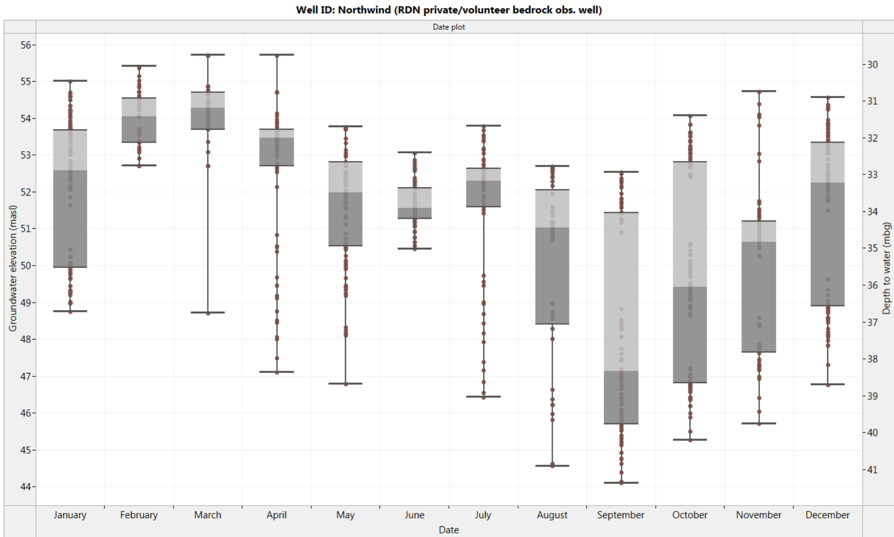
Figure 8. Northwind: Box and Whisker diagram for historical monthly groundwater level fluctuation (2013-2016)
