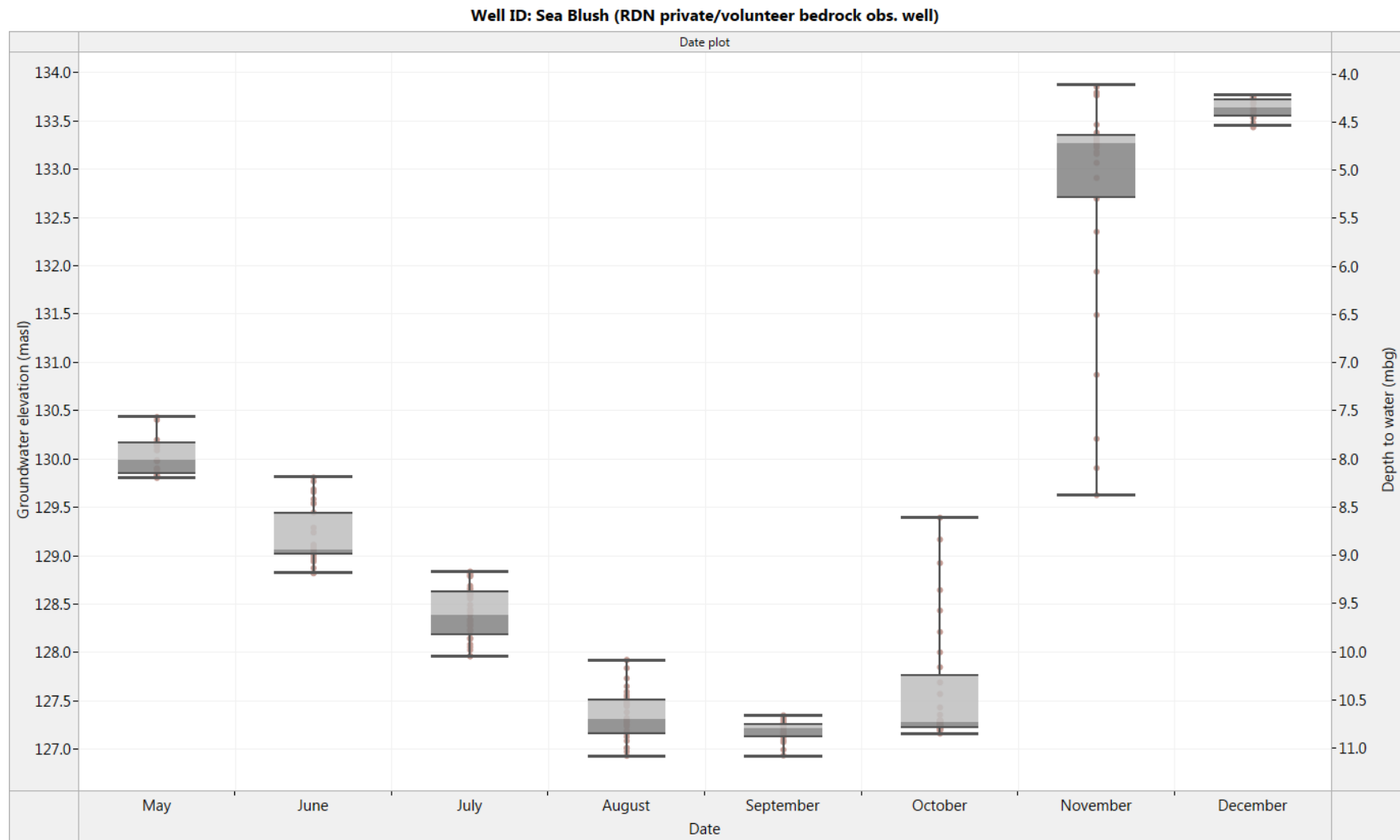
Figure 9. Sea Blush: Box and Whisker diagram for historical monthly groundwater level fluctuation (2016)
