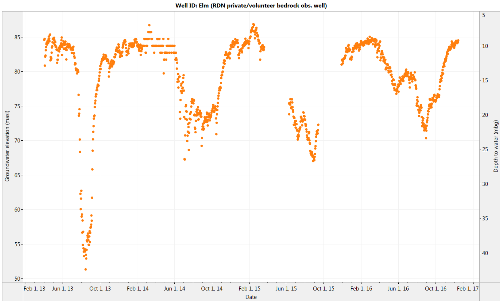
Figure 4. Elm: Historical water level (2013-2016)
