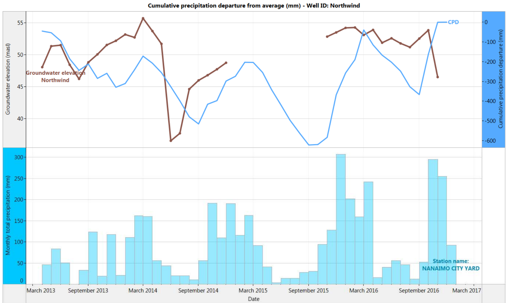
Figure 11. Northwind: Month end groundwater levels compared to cumulative precipitation departure curve and total monthly precipitation (2013-2016)
