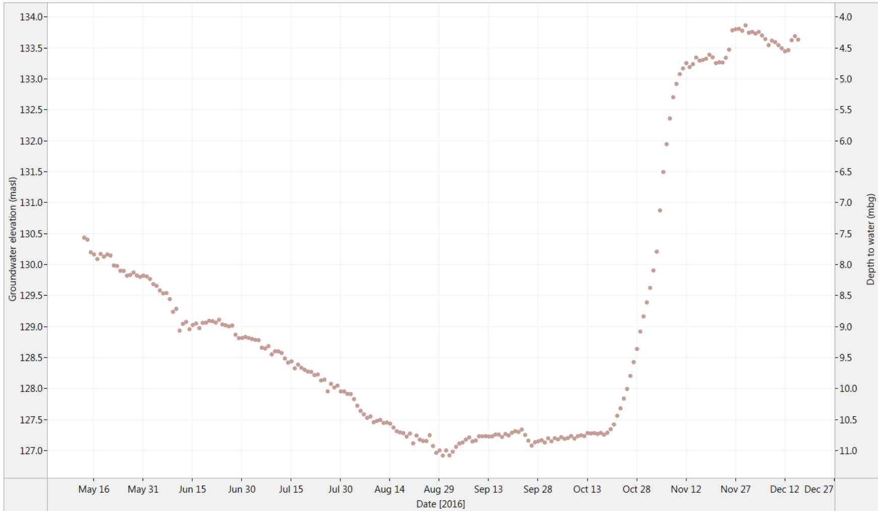
Figure 6. Sea Blush: Historical water level (2016)
