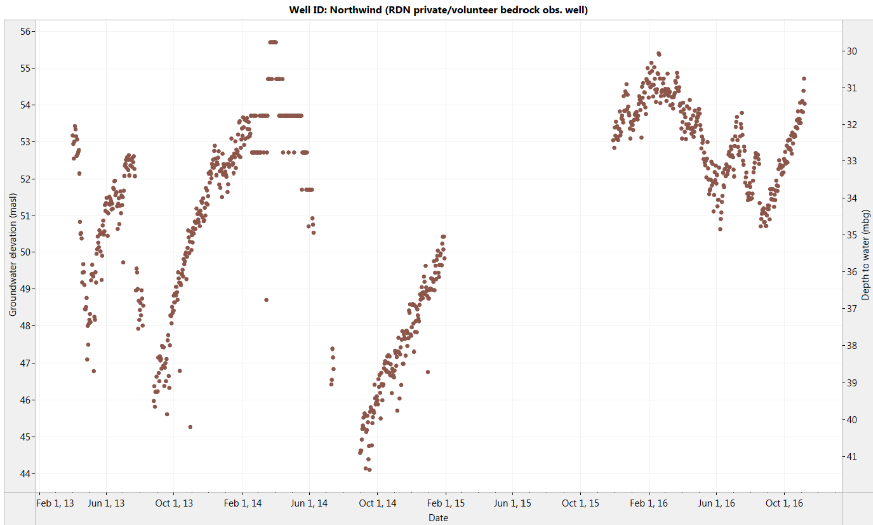
Figure 5. Northwind: Historical water level (2013-2016)
