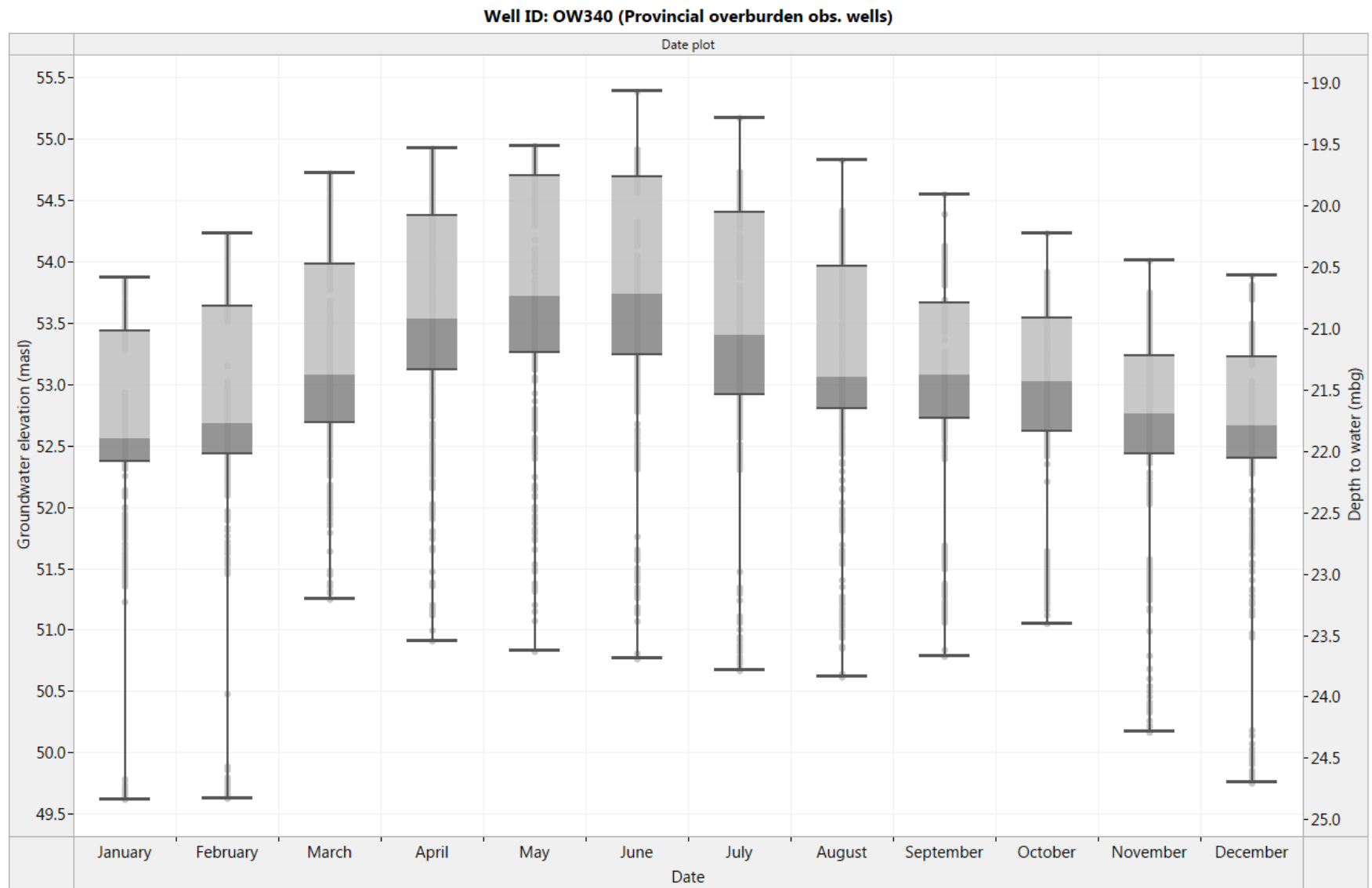
Figure 8. OW340: Box and Whisker diagram for historical monthly groundwater level fluctuation (1999-2016)
