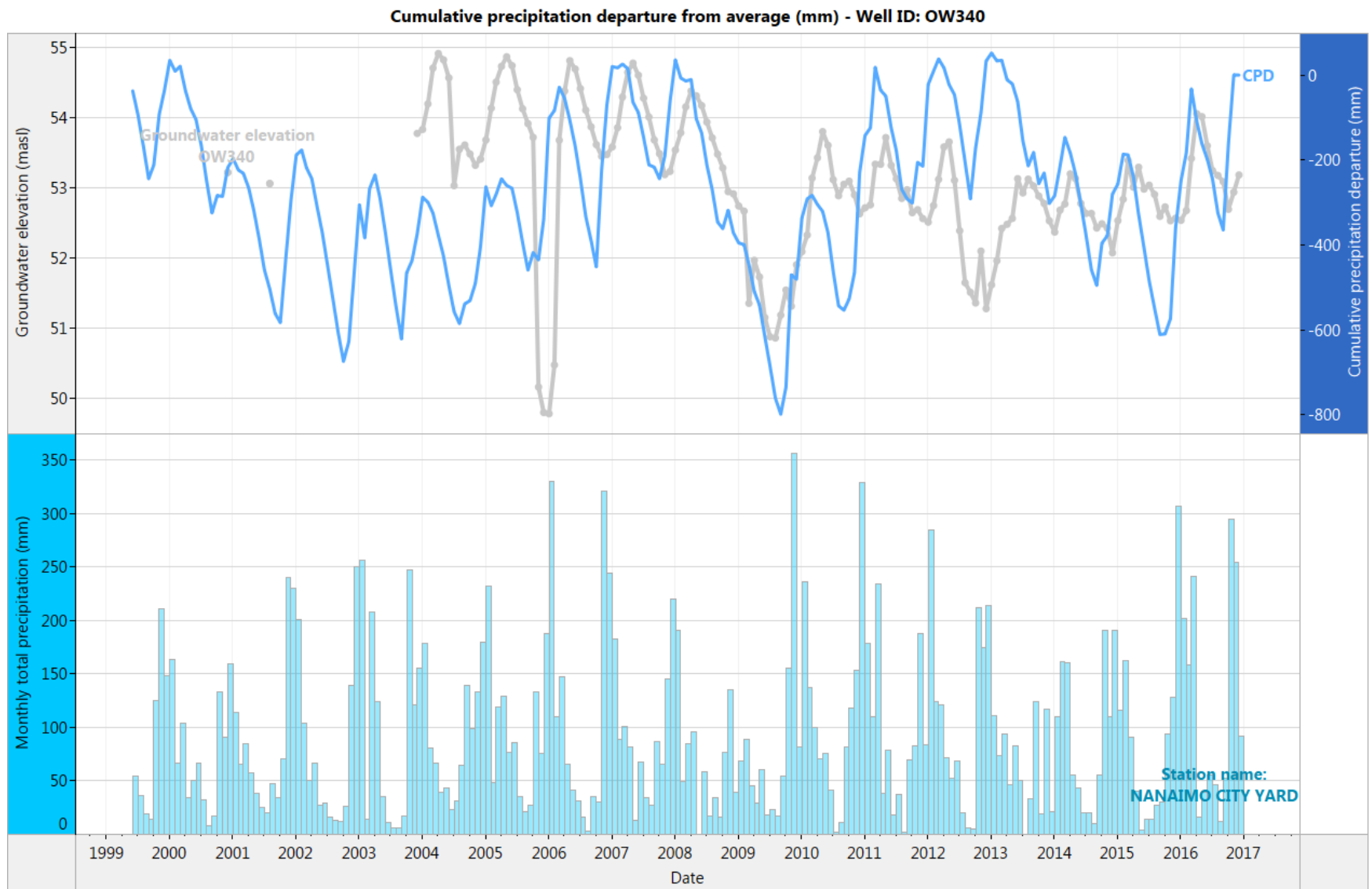
Figure 10. OW340: Month end groundwater levels compared to cumulative precipitation departure curve and total monthly precipitation (1999-2016)
