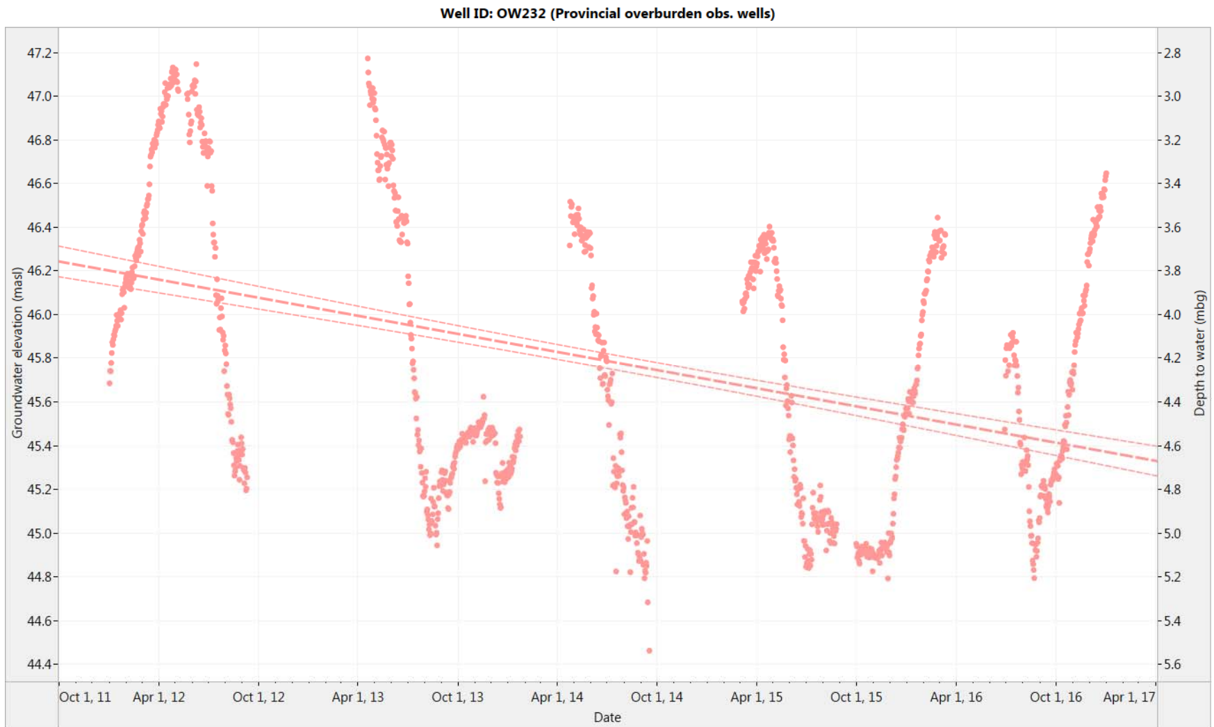
Figure 4. OW232: Water level and trend line estimation for the last five years (2012-2016)
