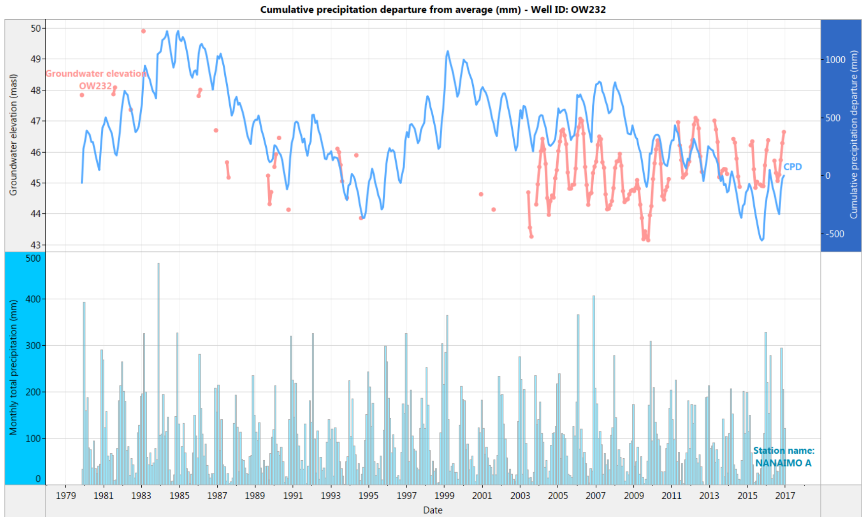
Figure 9. OW232: Month end groundwater levels compared to cumulative precipitation departure curve and total monthly precipitation (1979-2016)
