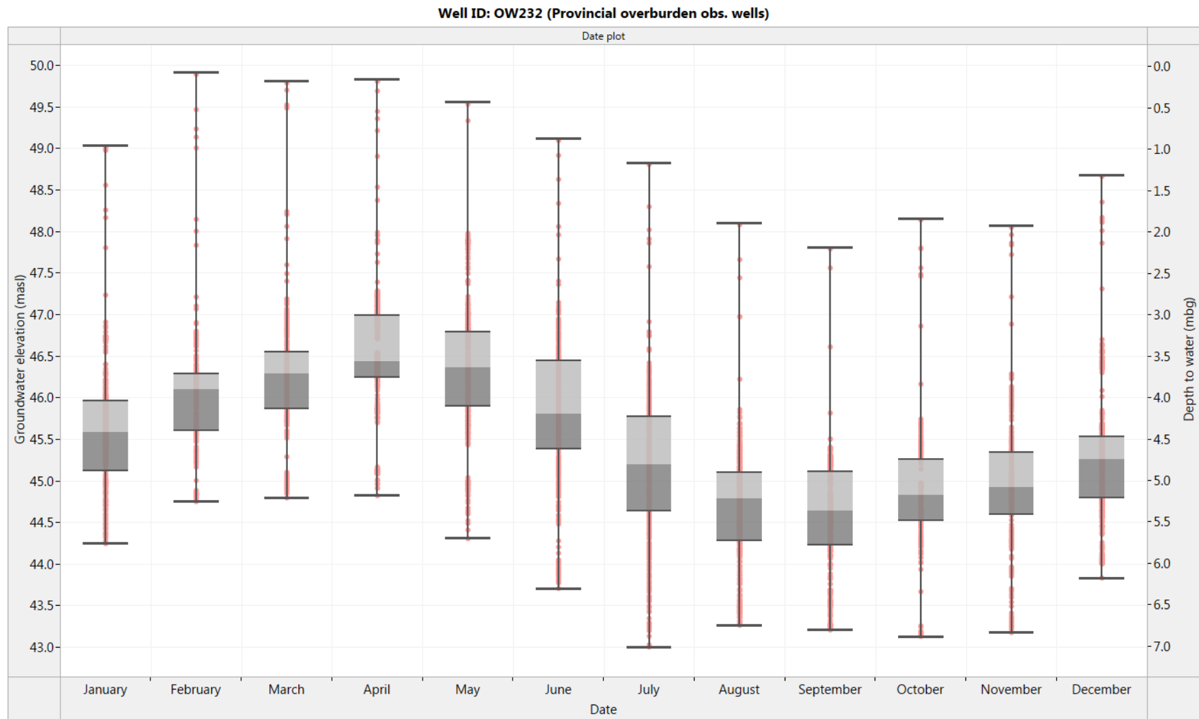
Figure 7. OW232: Box and Whisker diagram for historical monthly groundwater level fluctuation (1979-2016)
