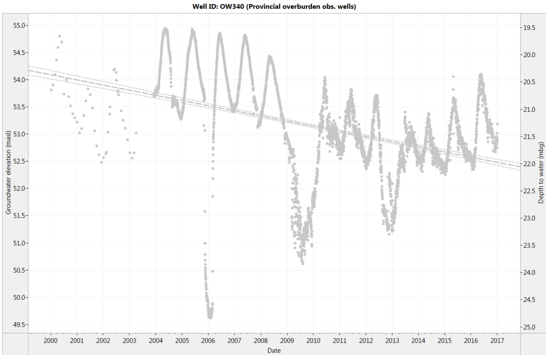
Figure 5. OW340: Historical daily water level (1999-2016) and trend line estimation (2000-2016)
