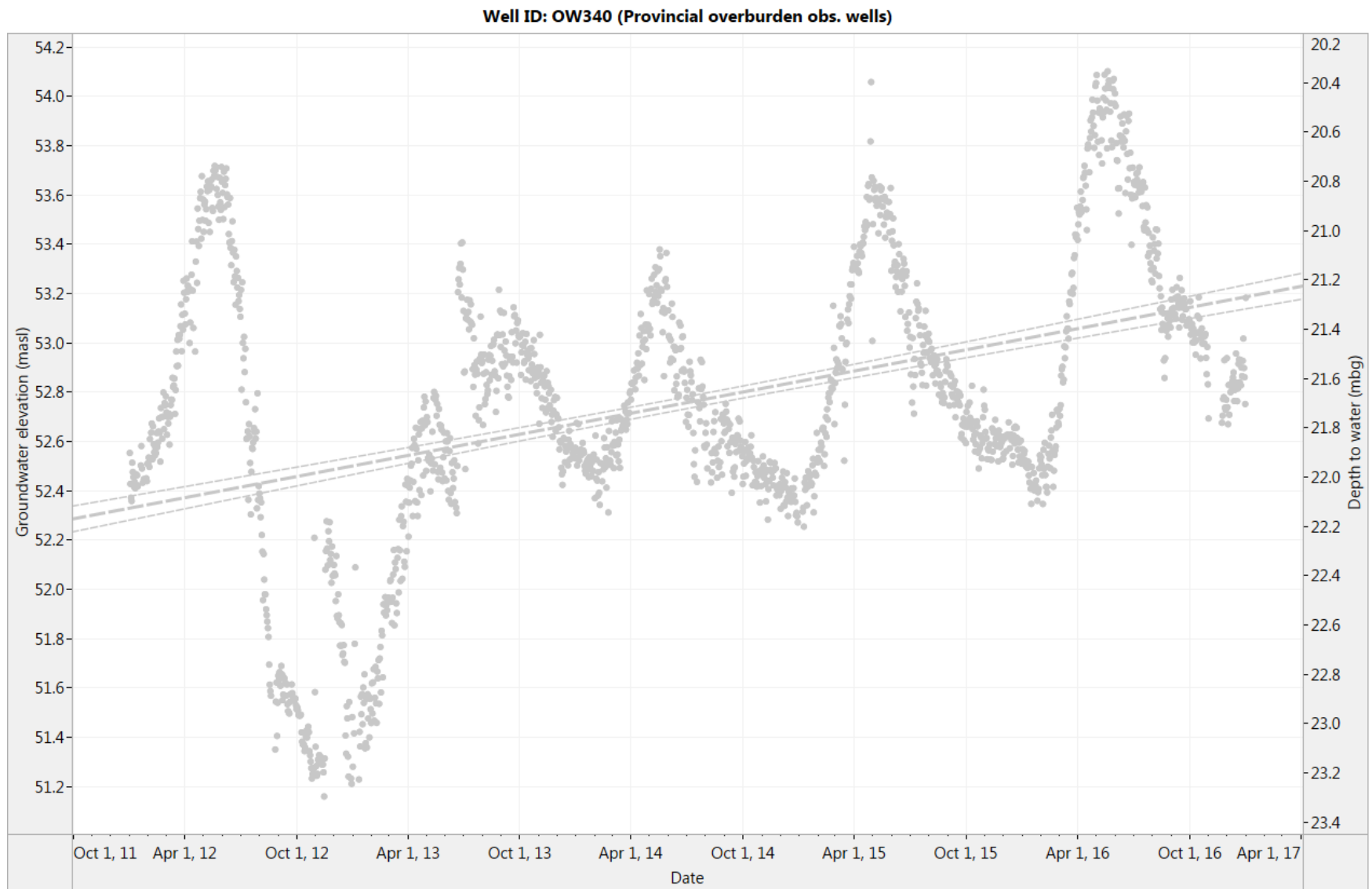
Figure 6. OW340: Water level and trend line estimation for the last five years (2012-2016)
