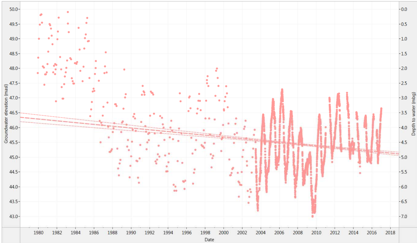
Figure 3. OW232: Historical daily water level (1979-2016) and trend line estimation (1979-2016)
