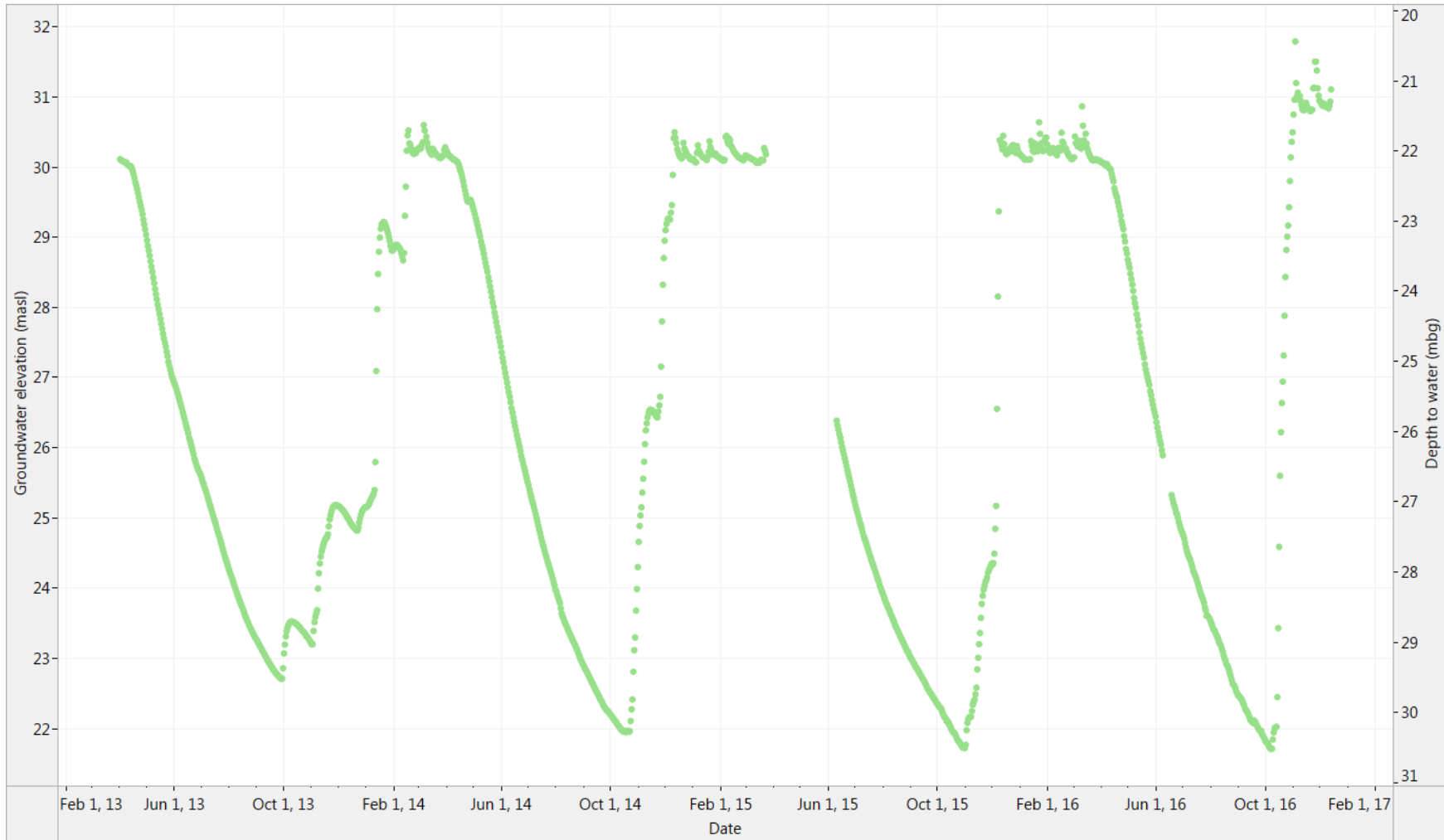
Figure 4. Grandom: Historical water level (2013-2016)
