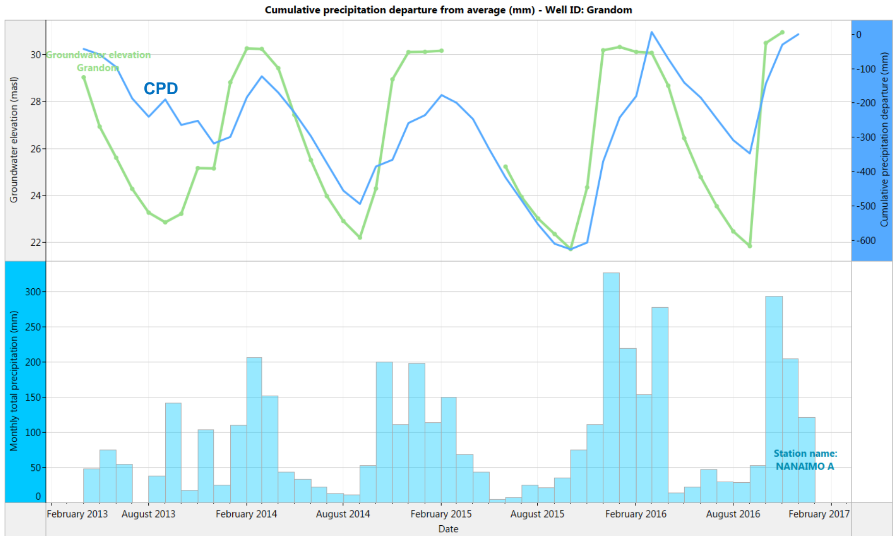
Figure 8. Gandom: Month end groundwater levels compared to cumulative precipitation departure curve and total monthly precipitation (2013-2016)
