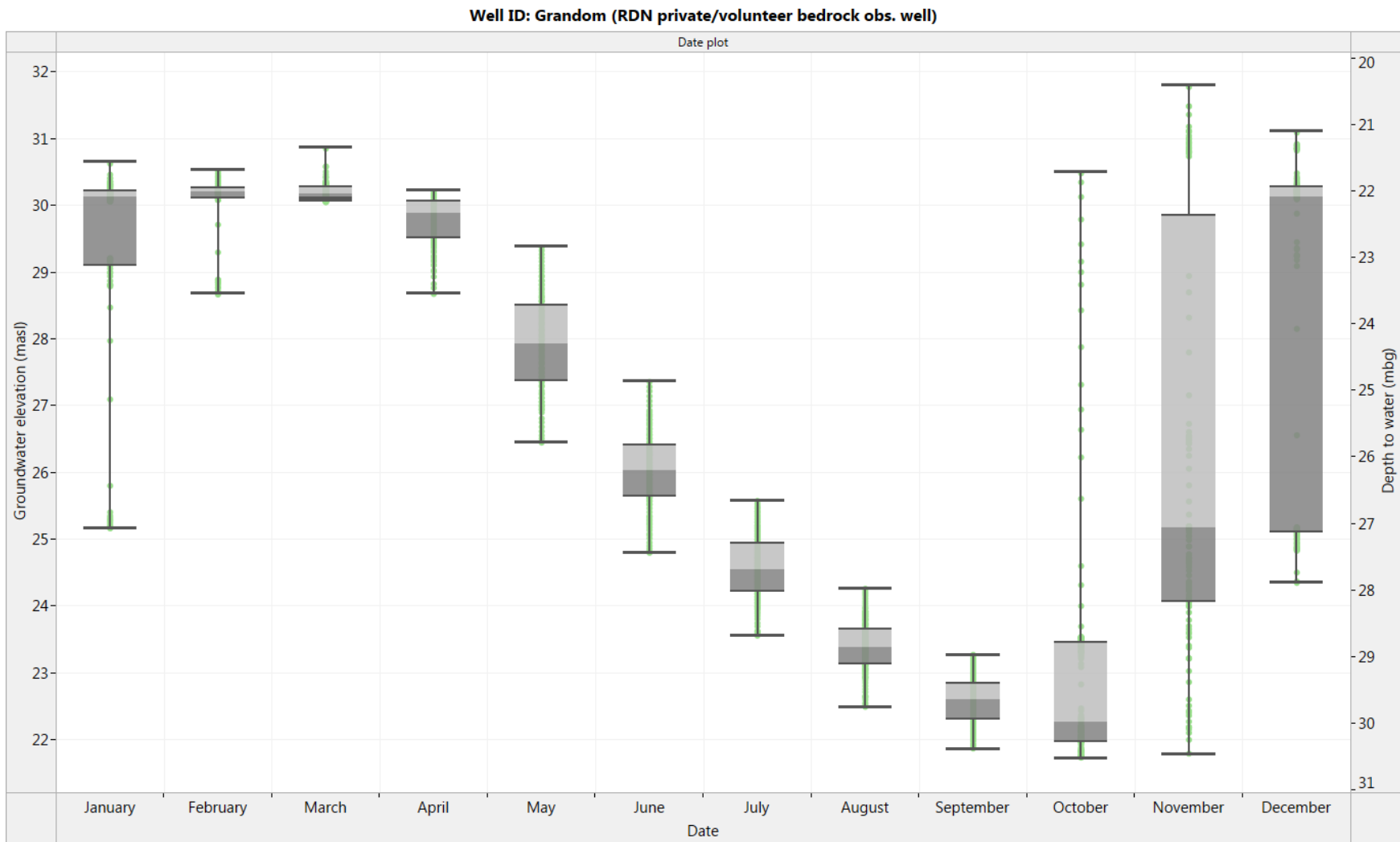
Figure 6. Gandom Box and Whisker diagram for historical monthly groundwater level fluctuation (2013-2016)
