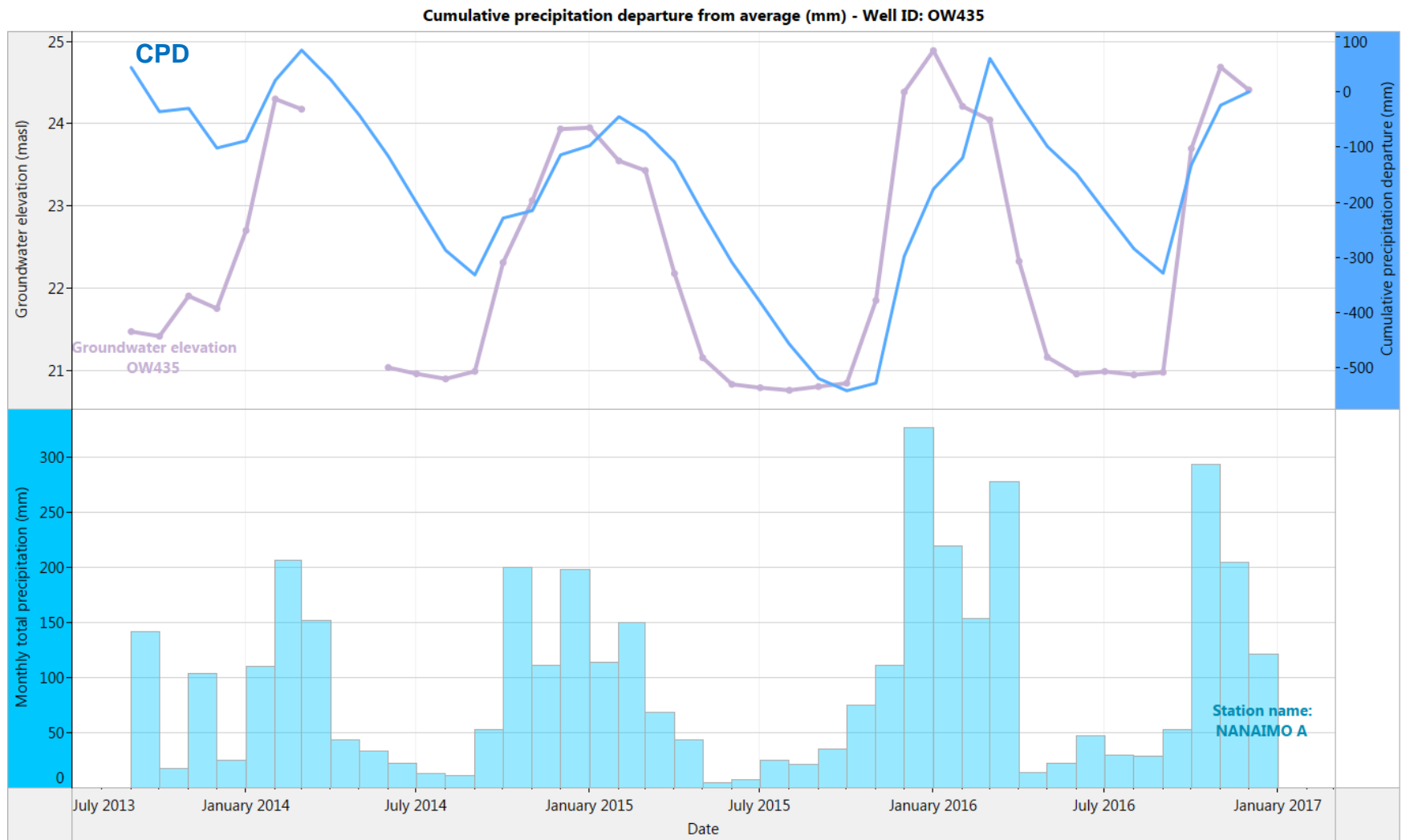
Figure 7. OW435: Month end groundwater levels compared to cumulative precipitation departure curve and total monthly precipitation (2013-2016)
