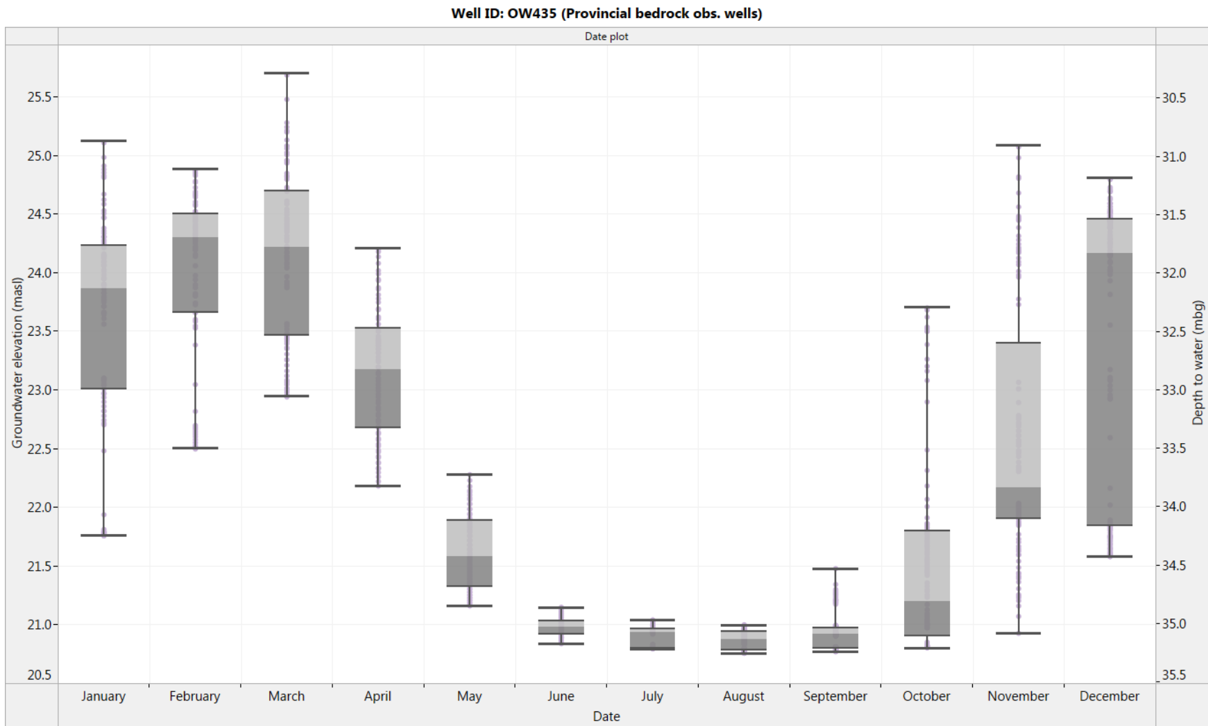
Figure 5. OW435: Box and Whisker diagram for historical monthly groundwater level fluctuation (2013-2016)
