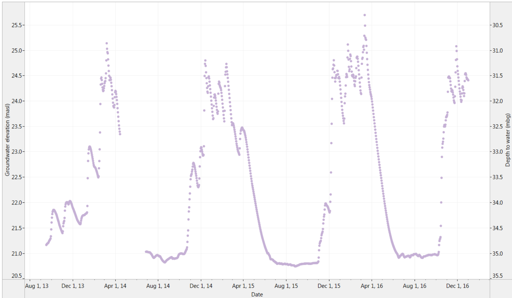
Figure 3. OW435: Historical water level (2013-2016)
