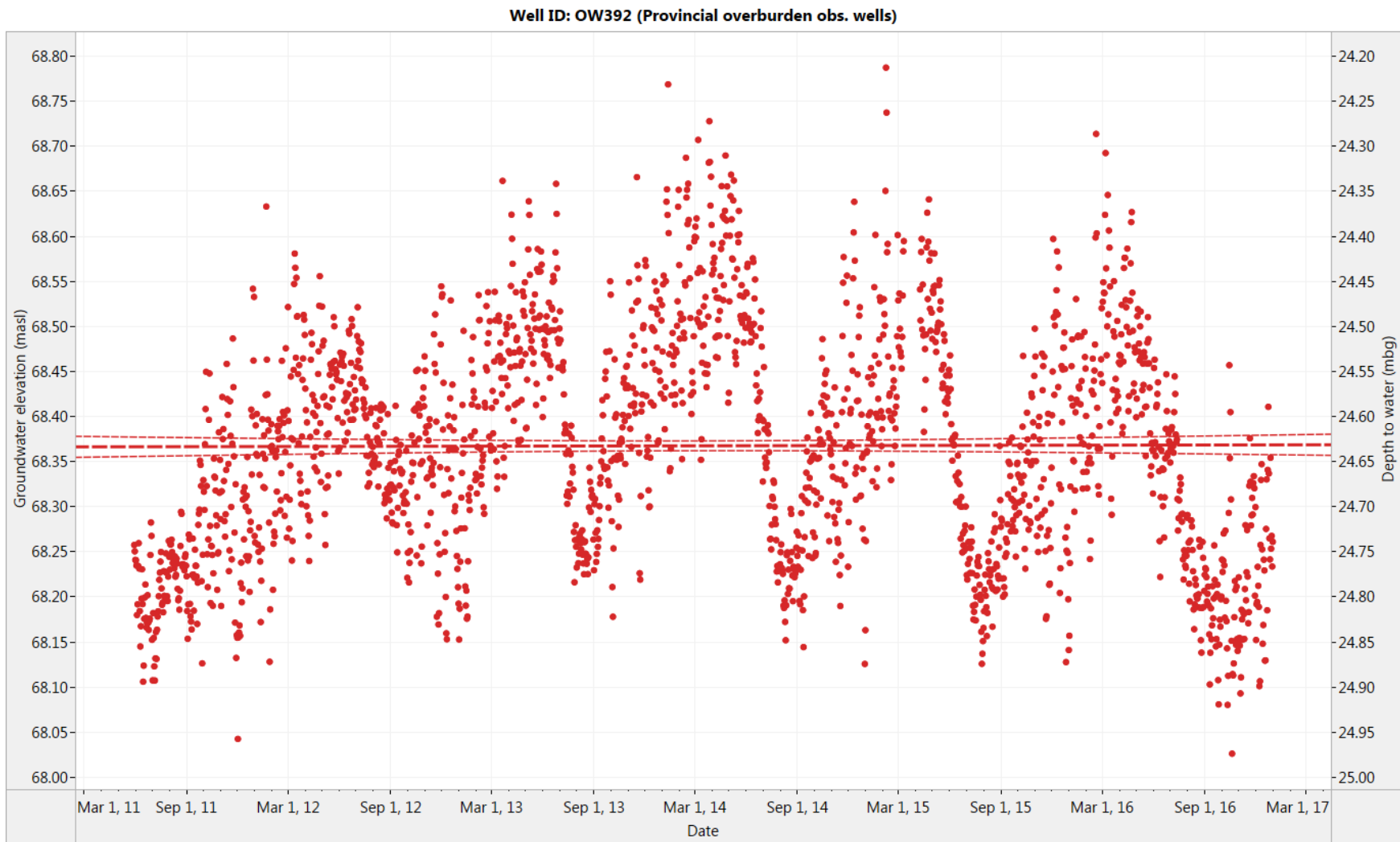
Figure 3. OW392: Historical daily water level (2011-2016) and trend line estimation (2012-2016)
