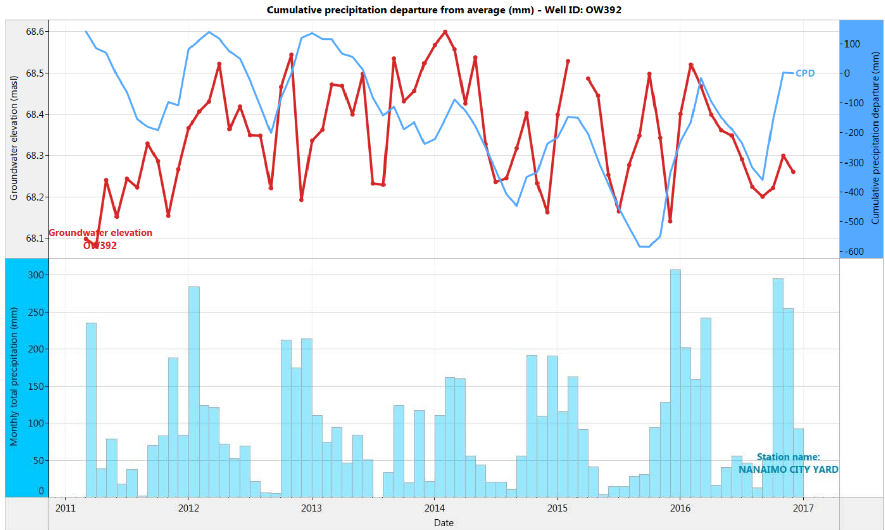
Figure 5. OW392: Month end groundwater levels compared to cumulative precipitation departure curve and total monthly precipitation (2011-2016)
