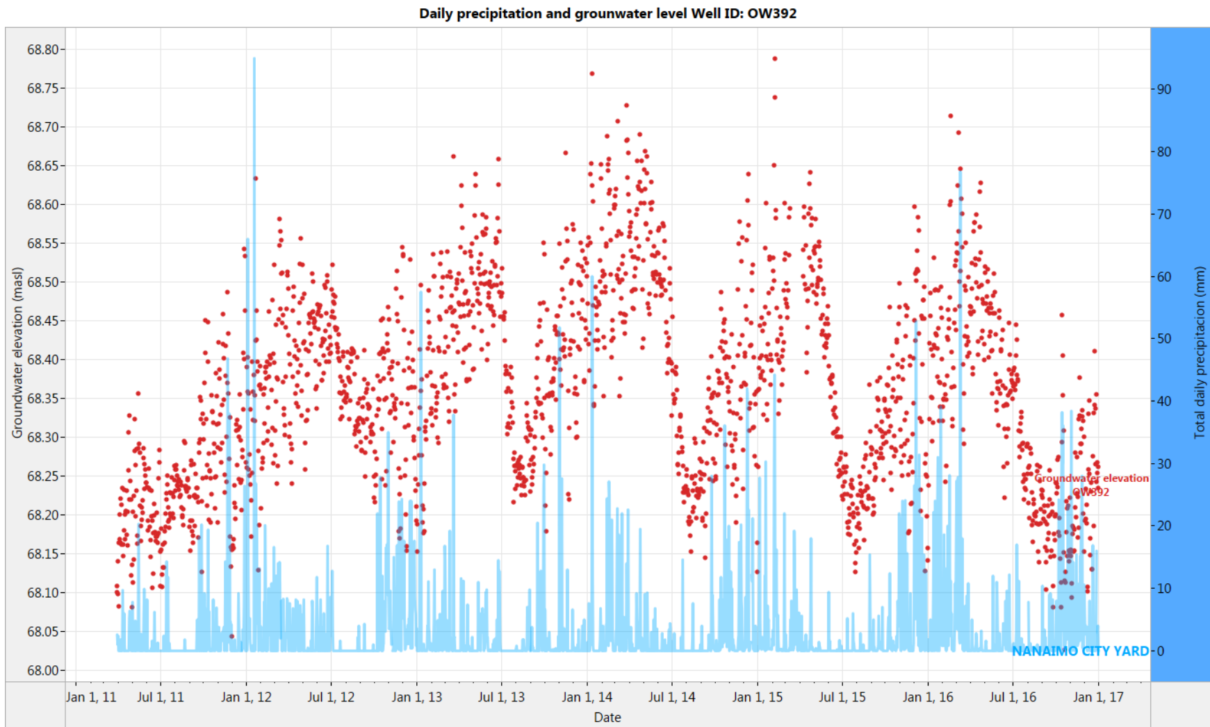
Figure 6. OW392: Daily groundwater levels compared to total daily precipitation (2010-2016)
