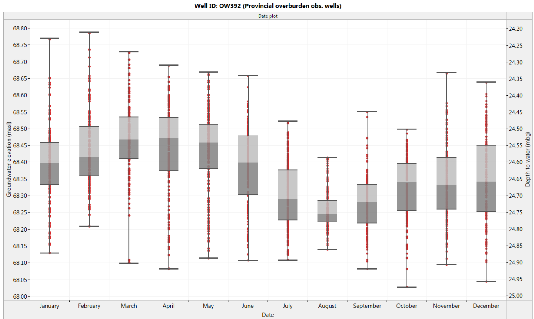
Figure 4. OW392: Box and Whisker diagram for historical monthly groundwater level fluctuation (2011-2016)
